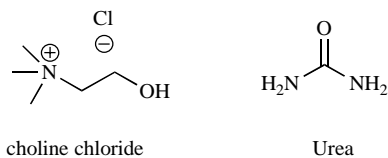
Fig. (11). Choline chloride and urea.
